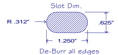
De-Burr all edges
