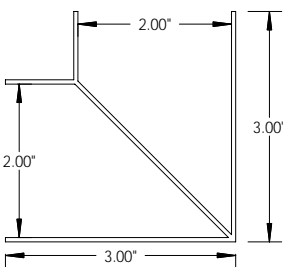
7719 2" Corner Channel
