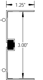
7910 3" Panel Adapter
