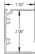
77122 2" Screen Channel
